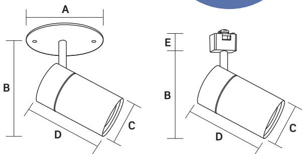
MONO-POINT
