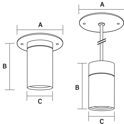
CEILING MOUNT
