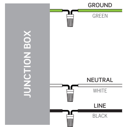
WIRING DIAGRAM 2
