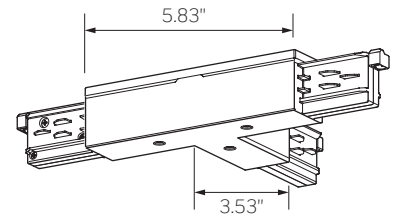
T-Couplers with Feeding Option
