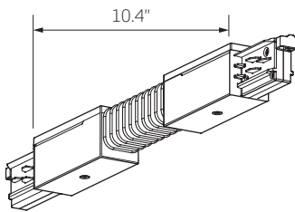
Flex Coupler with Feeding Option
