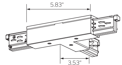
T-Couplers with Feeding Option
