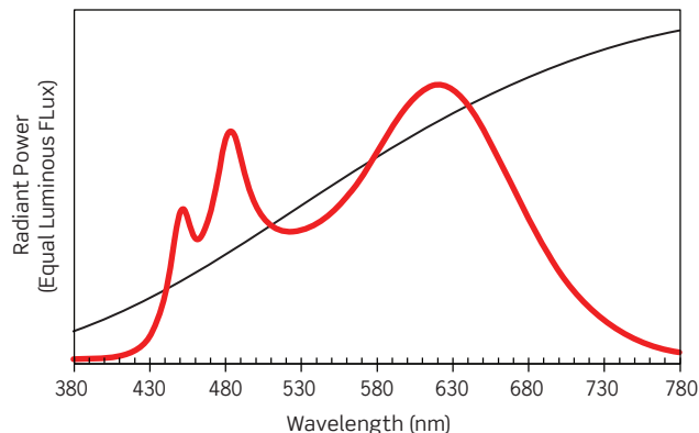
Spectral Power Distribution Comparison
