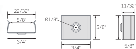
Mounting Clips
